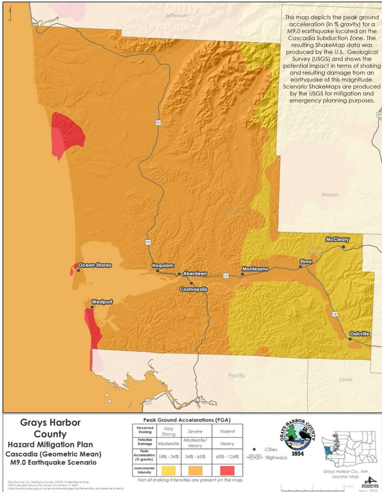
Figure 6-4 Cascadia M9.0 Fault Scenario
