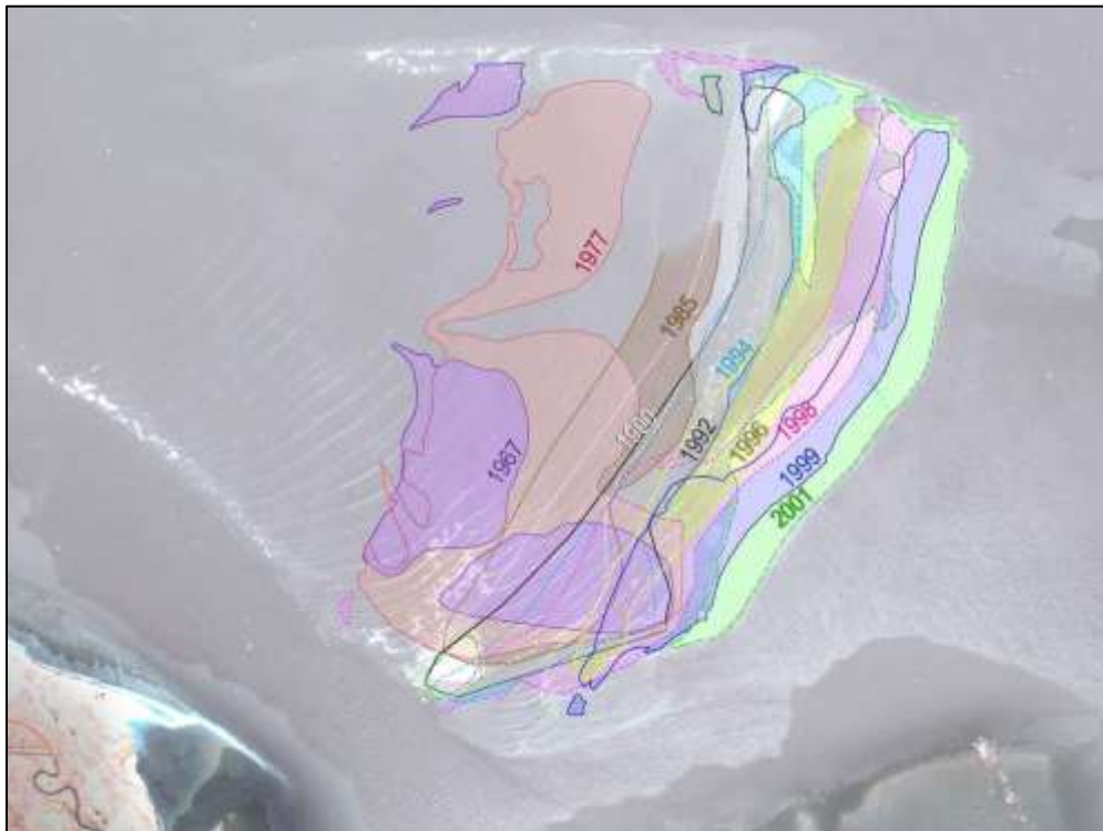
Figure 7-29 Eastward migration of Whitcomb Flats from 1967 to 2001 (from Osborne, 2003)
