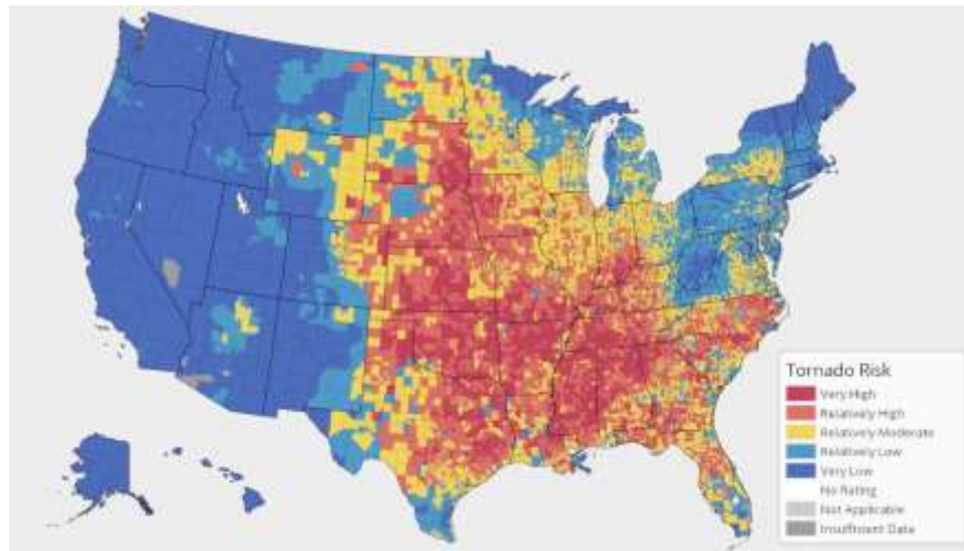
Figure 10-9 Tornado Risk Areas in the United States (2023)
