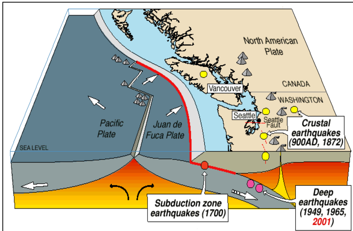
Figure 6-1 Earthquake Types in the Pacific Northwest
